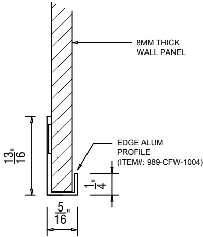
SECTION - A
