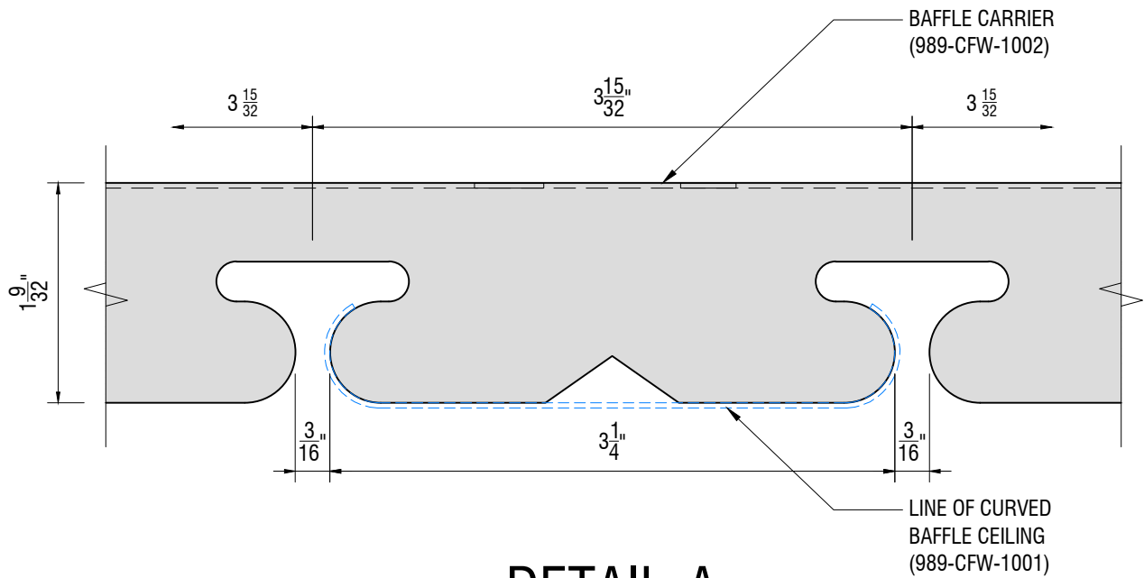
DETAIL-A
